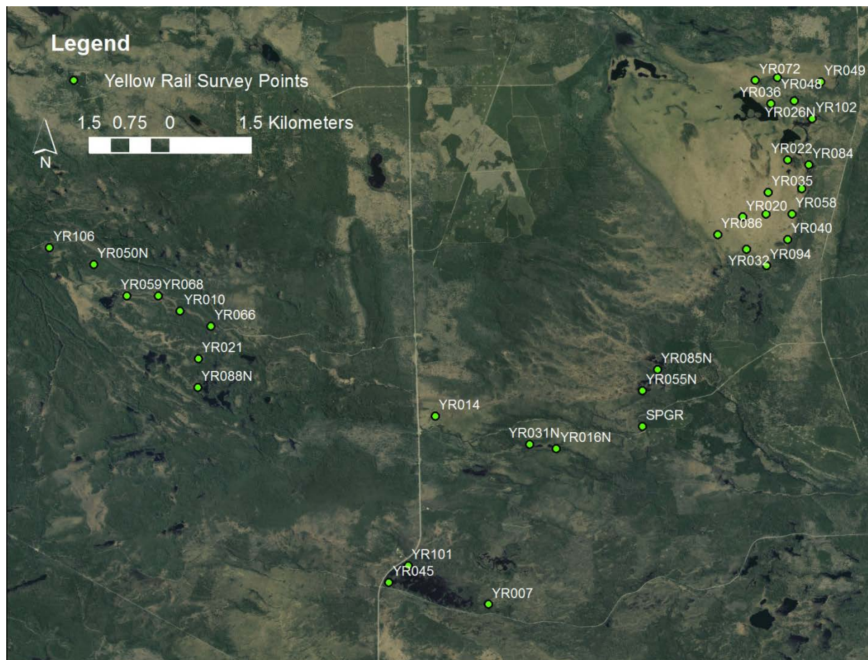
Figure 3. Points visited during Yellow Rail surveys conducted within Hiawatha National Forest in 2017.
